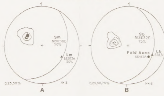
Figures 16A and 16B. A) Lower hemisphere equal area projection of poles to the mylonitic schistosity (S 2 ) at location V13 (P1.2) and associated shear band foliation (S 4 ) at location V13 (P1.2). B) Lower hemisphere equal area projection of poles to the (S 2 ) - Contour interval represents 5° of data per 18 area. Plane of best S 2 . Both fabrics contain a strong down-dip mineral lineation, and display a consistent east-over-west shear fabric parallel to that lineation. Thin mark denotes north direction that the fold axis lineation of the Phase Four folds is subparallel to it, suggesting that they were related during shear band development.
